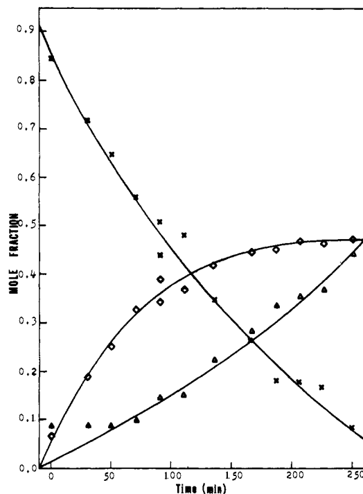
Figure 4. The mole fractions of intermediate A, \text{TMPFe}^{\text{OOFe}}\text{TMP} , intermediate B, \text{TMPFe}^{\text{IV}}\text{O} and \text{TMPFe}^{\text{III}}\text{OH} , during thermal decomposition of A in toluene solution at -30^\circ\text{C} : crosses, \text{TMPFe}^{\text{OOFe}}\text{TMP} ; squares, \text{TMPFe}^{\text{IV}}\text{O} ; triangles, \text{TMPFe}^{\text{III}}\text{OH} .
