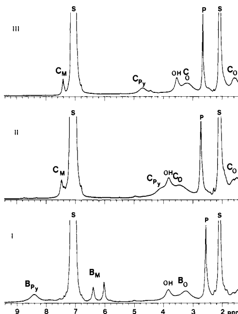
Figure 7. 360-MHz ^1\text{H} NMR spectra showing the effect of adding N -methylimidazole to intermediate B, \text{TMPFe}^{\text{IV}}\text{O} : trace I, a toluene solution of B ( \sim 4 mM) at -60^\circ\text{C} ; trace II, the same solution after the addition of 50\ \mu\text{L} (63 mM solution) of N -methylimidazole at -60^\circ\text{C} ; (N\text{-MeIm})\text{TMPFe}^{\text{IV}}\text{O} is present; trace III, the same solution at -30^\circ\text{C} . Resonance assignments: \text{Py} , pyrrole; m, meta-mesityl; o, ortho-mesityl methyl; p, para-mesityl methyl; s, solvent; OH, para-mesityl methyl of \text{TMPFeOH} .
