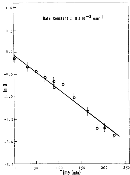
Figure 5. Plot showing first-order decay of intermediate A, \text{TMPFeOOFcTMP} , in toluene- d_8 at -30^\circ\text{C} .
