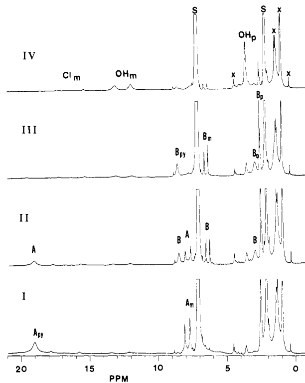
Figure 2. 360-MHz ^1\text{H} NMR spectra showing the thermal decomposition of \sim 4 mM TMPFeOOFeTMP in toluene- d 8 solution under 1 atm of dioxygen: trace I, intermediate A TMPFeOOFeTMP, at -30 °C; trace II, sample from I kept at -30 °C for 1 h; trace III, sample from trace II kept at -20 °C. Resonances due to individual species are denoted by capital letters: A, TMPFeOOFeTMP; B, TMPFeO; OH, TMPFeOH; Cl, TMPFeCl from incomplete reduction; S, solvent; X, impurities. Subscripts refer to resonance assignments as follows: py, pyrrole; m, meta-H; o, ortho-CH 3 ; p, para-CH 3 .
