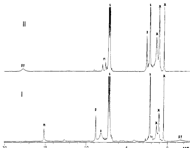
Figure 1. The 360-MHz 1 H NMR spectra of toluene- d 8 solutions at -70 °C of I, TMPFe II , II, TMPFe II + O 2 (1 atm), the species present in II is intermediate A, TMPFeOOFeTMP. Resonances are identified by the following symbols: py, pyrrole protons; m, meta-mesityl protons; o, ortho-mesityl methyl protons; p, para-mesityl methyl protons; S, residual undeuterated solvent; X, impurities in the solvent.
